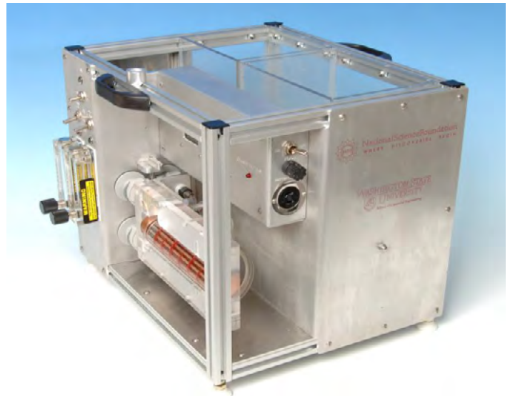
Figure 1. Second generation Desktop Learning Module (DLM) with inserted shell and tube heat exchanger cartridge
